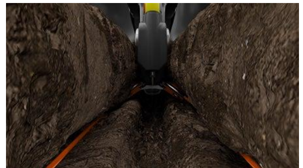
Figure 2. FurrowJet® Wing Placement
